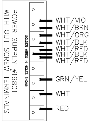
POWER SUPPLY DETAIL
