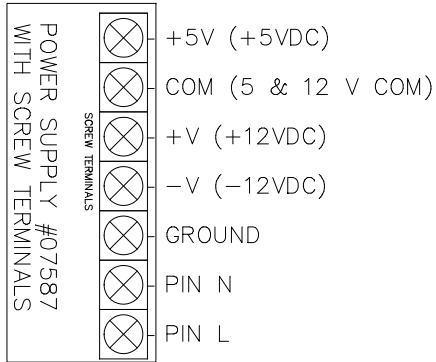
POWER SUPPLY DETAIL
