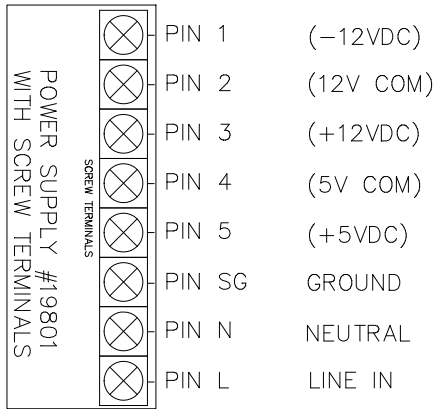
POWER SUPPLY DETAIL
